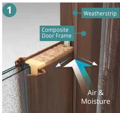
Weatherstrip is engineered in a variety of profiles to provide the best possible fit with our door systems, helping to deliver a precise seal between the door and frame . In addition, a rot-free Therma-Tru composite door frame* delivers extra protection from the damaging effects of moisture.
