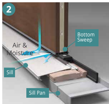
Sill and bottom sweep form a tight seal against wind-driven moisture infiltration at the bottom of the door system and help channel moisture away from the home. Sill pan (recommended) adds an extra layer of protection to help keep moisture away from the subfloor.
