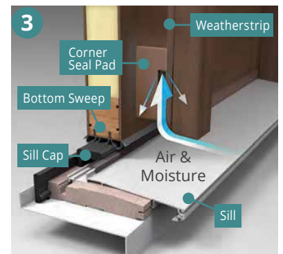
Corner seal pads (inswing only) complete the seal between the sill cap , bottom sweep and weatherstrip to help block potential pathways where wind-driven moisture can infiltrate the bottom corner of the door system.
