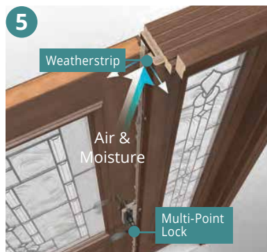
Multi-point locking system (recommended) engages the door and frame at three points from top to bottom for enhanced security while helping to preserve the seal of the weatherstrip even under wind pressure.
